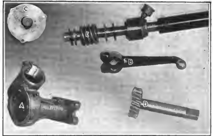
Fig. 4—Steering details: A, box; B, drop arm; C, cover; D, sector; E, shaft and worm
